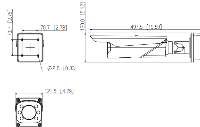
Dimensions (mm [inch])
